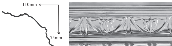
Holland Cornice 135mm x 1800mm L Ceiling Projection 110mm Wall Depth 75mm
