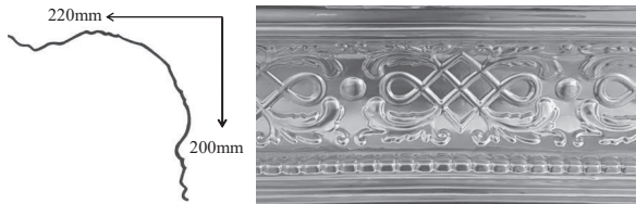
Baird 300mm x 1000mm L Ceiling Projection 220mm Wall Depth 200mm
