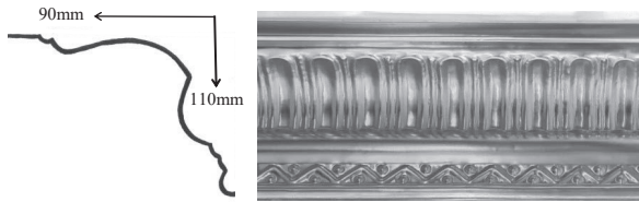
Accolade 160mm x 1800mm L Ceiling Projection 90mm Wall Depth 110mm
