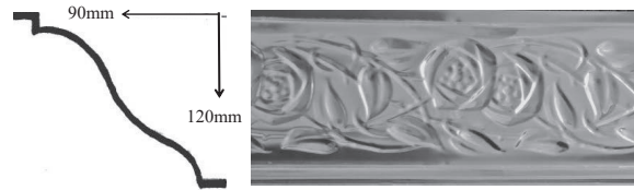
Rose Cornice 140mm x 1800mm Ceiling Projection 90mm Wall Depth 120mm
