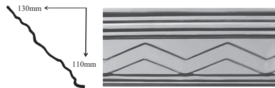
Pacific Cornice 150mm x 1800mm Ceiling Projection 130mm Wall Depth 110mm
