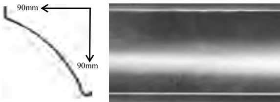
Plain Cornice 100mm x 1800mm Ceiling Projection 90mm Wall Depth 90mm
