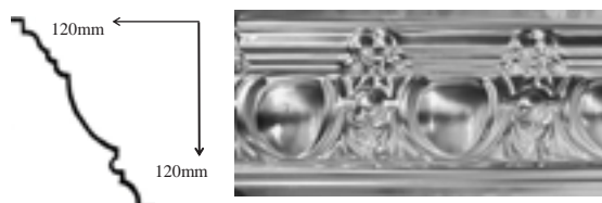
Egg and Dart Large (or Egg & Grape) 185mm x 1800mm L Ceiling Projection 120mm Wall Depth 120mm
