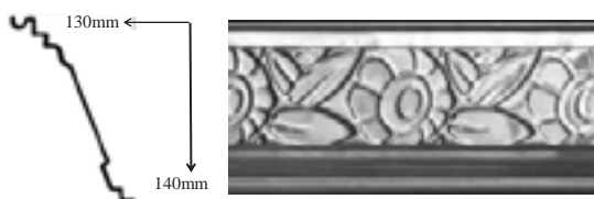
Clarence Cornice 160mm x 1800mm L Ceiling Projection 130mm Wall Depth 140mm
