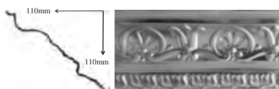
Commonwealth Cornice 150mm x 1800mm L Ceiling Projection 110mm Wall Depth 110mm
