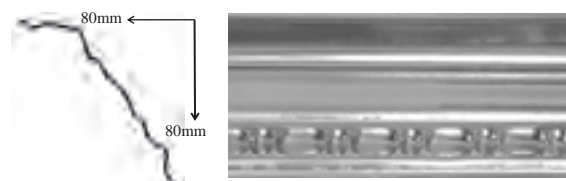
Lambton Cornice 110mm x 1800mm L Ceiling Projection 80mm Wall Depth 80mm
